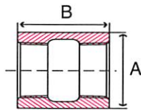
Fig. S3014CP & S3016CP - Full Coupling
