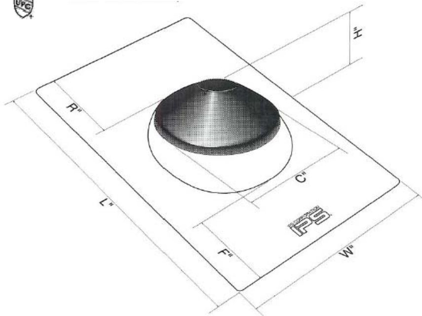
Roof Vent Flashing Dimensional Characteristics
