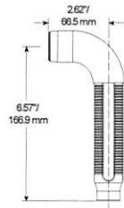
Long 90° elbow reducer
